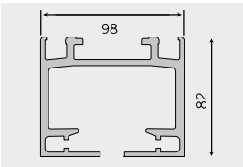
R-type track Track system for right-angled configurations with cross-roller carriers.
