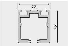
G-type track Mechanically coded junction technology with curves and switches.
