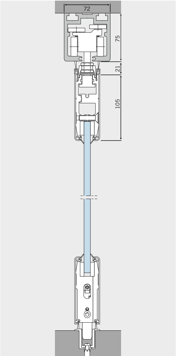
Basic Straightline element without support profile
